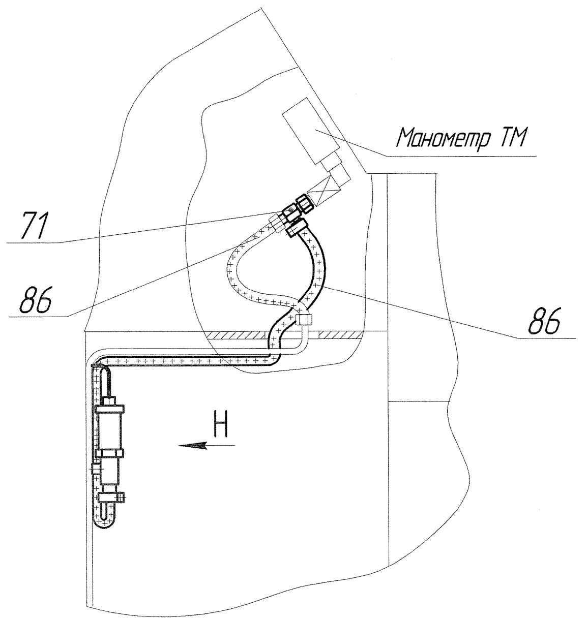
K (1:5) (1)
